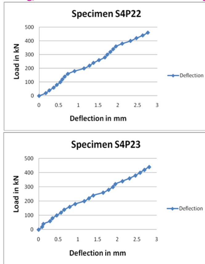
Figure7: Load-Displacement Curve for Specimens
